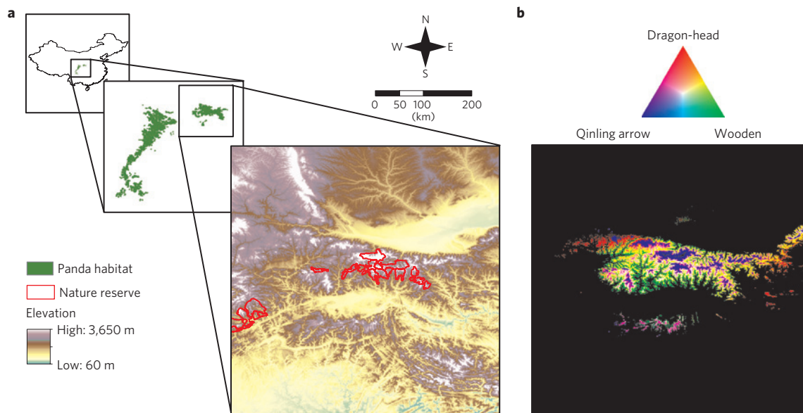
Figure 1 | Location and topography of the study area, and the baseline CSAs for the three bamboo species studied. a , The study area includes the Qinling Mountains and surrounding areas ( 5^\circ \times 5^\circ ). b , The CSAs for the Qinling arrow, dragon-head and wooden bamboos were obtained from the bioclimatic models under the baseline climate, and blue, red and green colours indicate the CSAs for the three species, respectively. The mixtures of the three colours indicate overlaps of the CSAs for individual species. The brightness of the colours shows the number of bioclimatic models (among the ten models with different presence data partitions) predicting pixels as suitable for each species, with brighter colours indicating a larger number of models.
